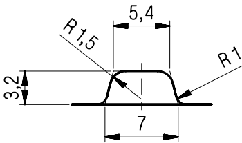
DETAIL CRAN Ech 2:1
